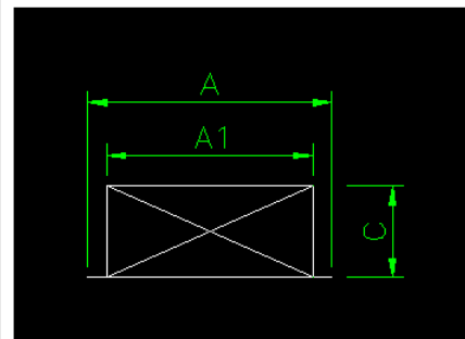
Flush-mounted cabinet
